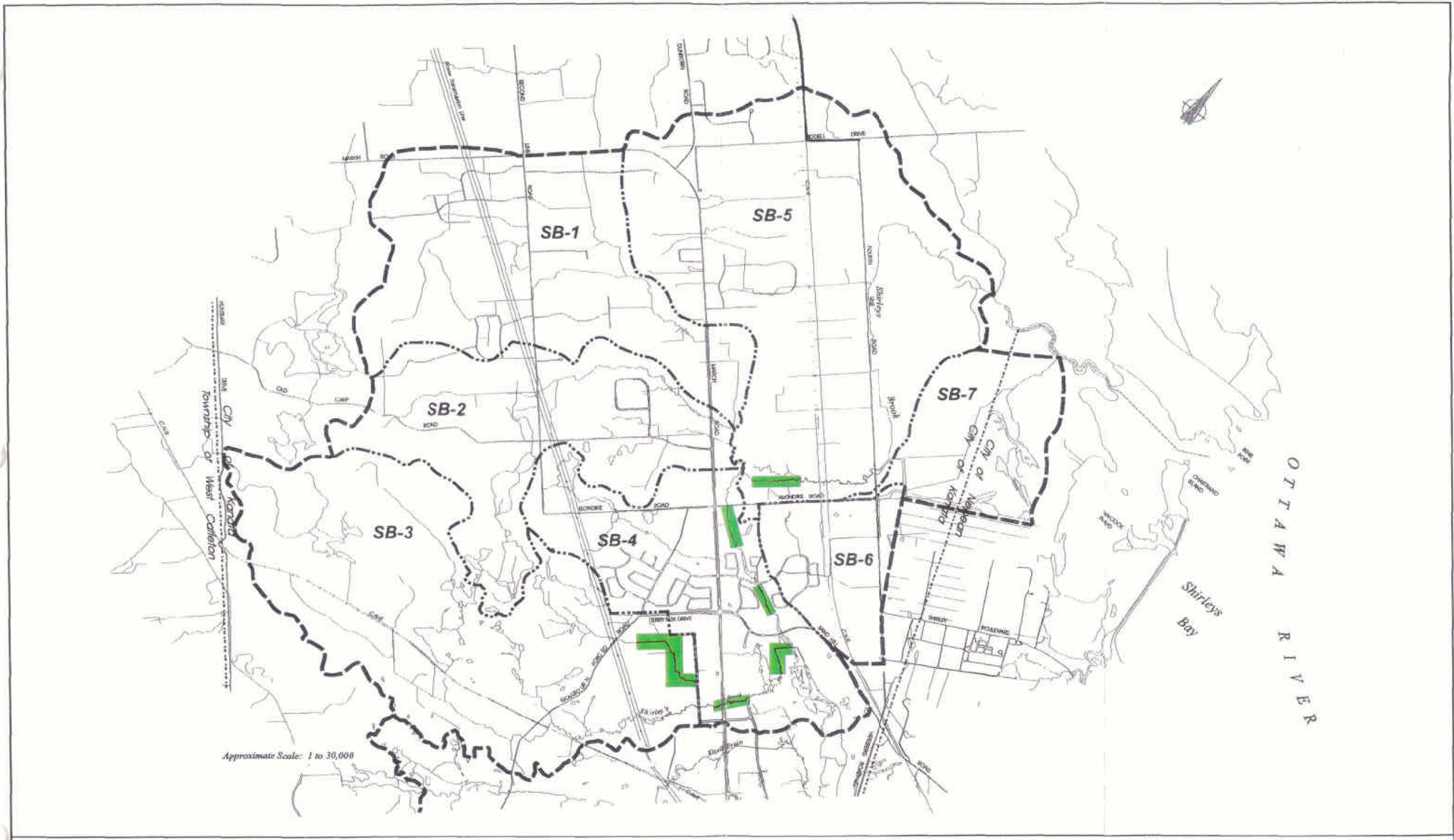
Shirley's Brook Subwatershed Proposed Channel Restoration Locations
